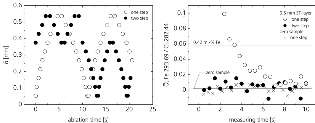
Fig. 7 Radial displacement R (left) of the laser beam as a function of time during the ablation phase and the resulting line ratio \tilde{Q}_{Fe} values during the measurement phase (right). Open symbols denote the one step ablation scheme, filled symbols denote the two-step scheme, see Fig. 6. For each data point shown in the right diagram an ablation sequence of 20 s was preceding as shown on the left.
