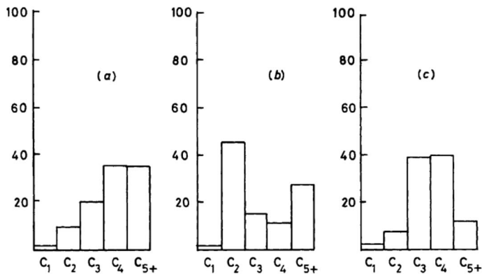
Fig. 7 Comparison of the product selectivities for the reaction of methanol and methylating agents over H-ZSM-5 at 250 °C. (a) \text{CH}_3\text{OH} (WHSV 0.005 \text{ h}^{-1} , 87% conversion), (b) (\text{CH}_3)_2\text{SO}_4 (WHSV 0.075 \text{ h}^{-1} , conversion 21%), (c) \text{CH}_3\text{I} (WHSV 0.06 \text{ h}^{-1} , conversion 0.1%). Reproduced with permission from ref. 25.
