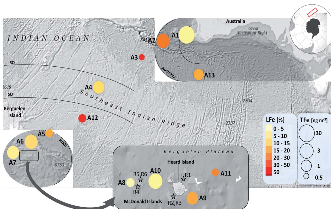
Fig. 3 Measurement of the total concentration, T_{Fe} ( ng\ m^{-3} , point size), and labile fraction, L_{Fe}\% (colour scale), of Fe in aerosols collected during the HEOBI campaign. Aerosol samples A1–A13 are represented by their mid-sampling location. L_{Fe}\% equals to 54 and 52% for A3 and A12, respectively. Samples A8–A11 were collected whilst the research vessel circumnavigated both islands. Rock sample ( R_x ) locations are indicated with grey stars. The dashed black lines and grey shading illustrate dominant aeolian influence found in aerosols, either volcanic emissions from Heard Island volcano, air mass issued from long-range transport over the SO or Australian dust and anthropogenic combustion particles.
