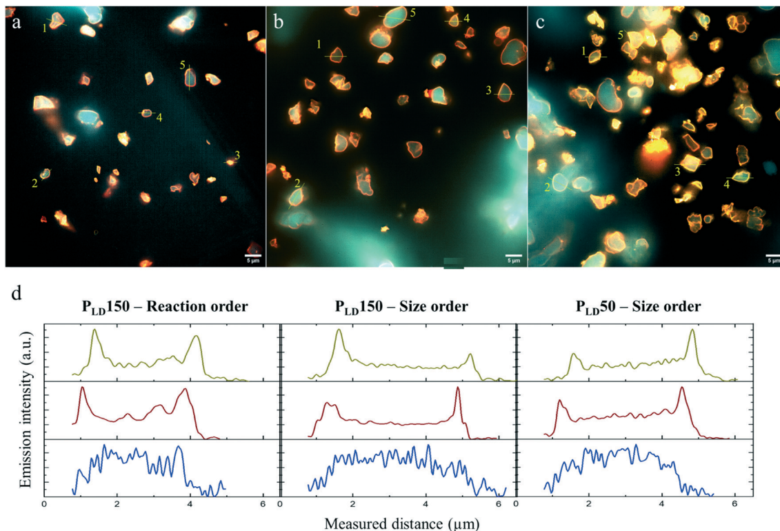
Fig. 4 The co-distribution of FateDH-Cy3, FaldDH-Cy5 and ADH-AF488 in MCF particles after the co-immobilization. Each image is a composite of the emission of the three dyes (Fig. S4, S6 and S8 † ). The scale bar is 5 \mu\text{m} . (a) P_{LD150} in reaction order, (b) P_{LD150} in size order, (c) P_{LD50} in size order. (d) Emission intensity profiles of particle #1 in a–c; Cy3 is shown in yellow, Cy5 in red, AF488 in blue. All the profiles are in Fig. S5, S7 and S9 † .
