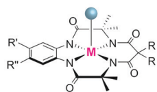
Chart 9 Summary of features of water oxidation catalysts with macrocyclic ligands.
