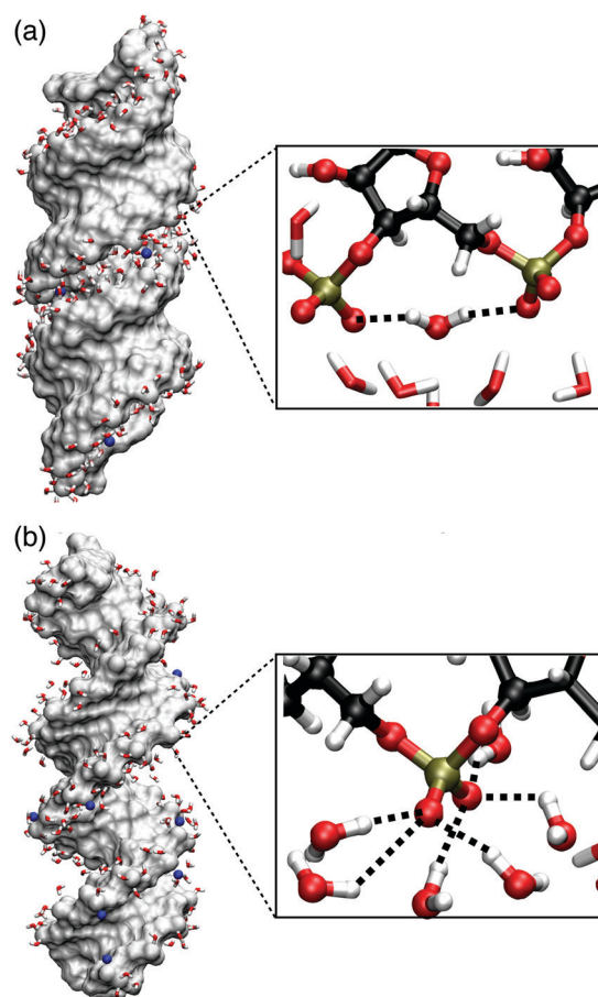
Fig. 11 Molecular surface of (\text{AU})_{23} dsRNA (a) and (\text{AT})_{23} DNA (b) for structures obtained from MD simulations (ref. 75) with \text{Na}^+ counterions shown in blue. The inlays show instantaneous hydration structures of the (\text{PO}_2)^- groups, highlighting a (\text{PO}_2)^- \cdots (\text{PO}_2)^- bridging water molecule (a) and local hydration structures of six water molecules forming HBs with one (\text{PO}_2)^- groups (b).
