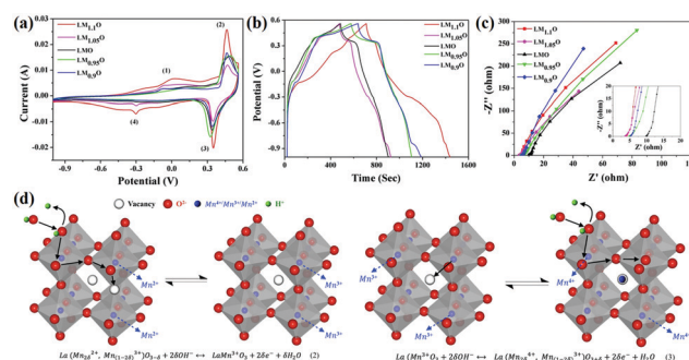
Fig. 6 (a) Cyclic performance of the \text{LM}_{1\pm x}\text{O}_3 samples at a scan rate of 0.01 \text{ V s}^{-1} . (b) Charge-discharge curves in a potential window of -1 to 0.56 V at 1 \text{ A g}^{-1} . (c) EIS of the \text{LM}_{1\pm x}\text{O}_3 samples with the inset of enlarged R_s at high frequencies. (d) Charge storage mechanism in \text{LM}_{1\pm x}\text{O}_3 perovskite oxide materials. Reproduced from ref. 91 with permission from Elsevier B.V., copyright 2017.
