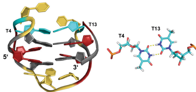
Fig. 4 Chair-type anti-parallel G-quadruplex of the TBA aptamer d(GGTTGGTGTGGTGG) in K + solution (110 mM KCl, pH 6.1) and hydrogen-bonded base pair formed between two T residues from opposite T-T lateral loops (PDB 148D); 46 anti - and syn -Gs of the quadruplex core, loop residues, and the T-T base pair are colored grey, red, yellow, and cyan, respectively.
