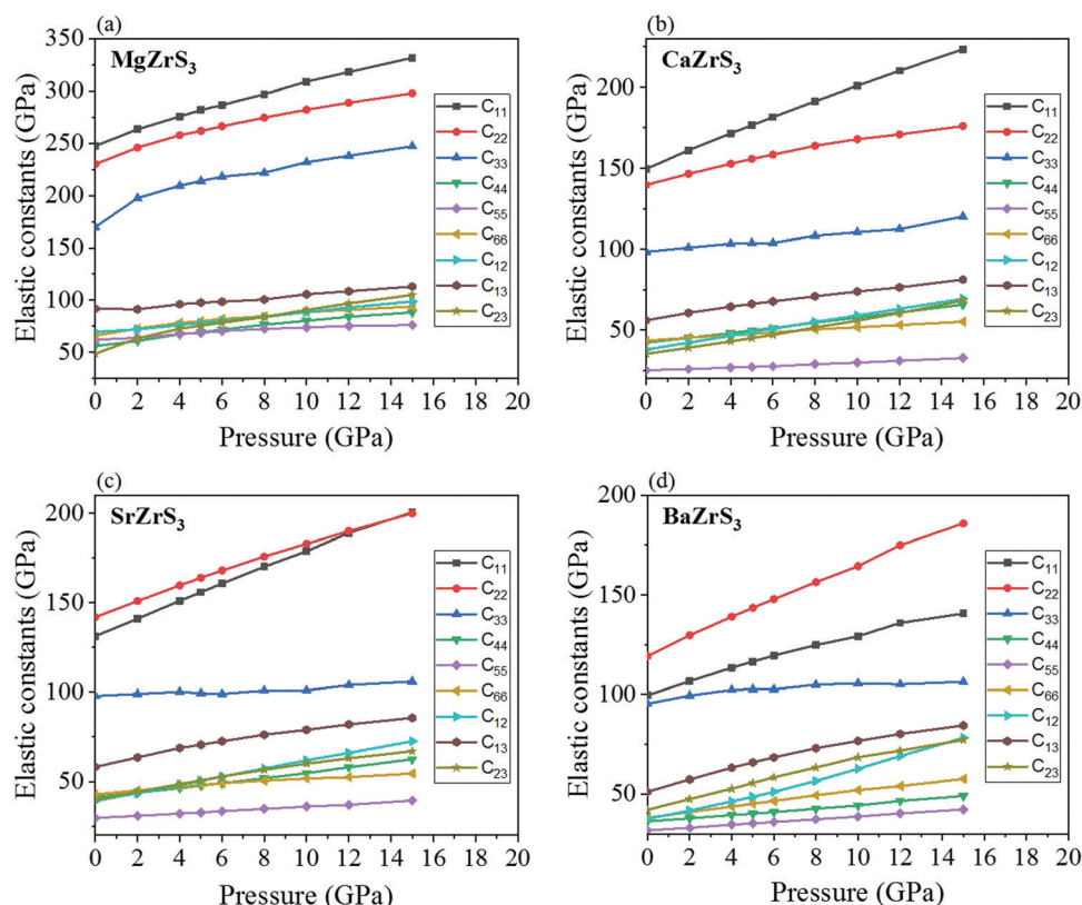
Fig. 3 Elastic constants vs. pressure for (a) \text{MgZrS}_3 , (b) \text{CaZrS}_3 , (c) \text{SrZrS}_3 , and (d) \text{BaZrS}_3 .
