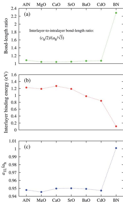
Fig. 2 Structural features of the h-MgO structure in contrast to those of h-BN. (a) Ratios of the interlayer distance ( c_{hL}/2 ) to intralayer bond length ( a_{hL}/\sqrt{3} ). (b) Interlayer binding energies, defined as monolayer-to-bulk total energy difference per cation-anion pair. (c) Monolayer-to-bulk lattice parameter ratios ( a_{1L}/a_h ).
