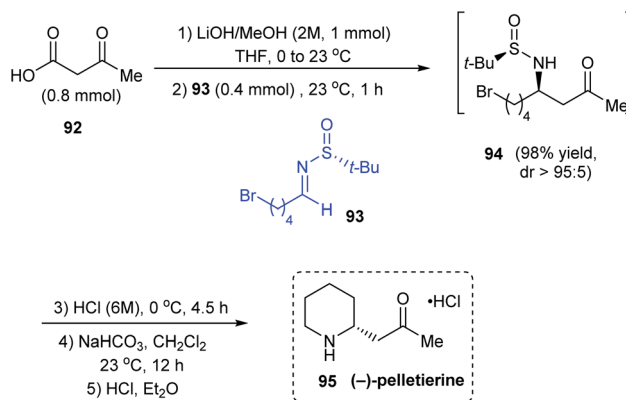
Scheme 17 Synthesis of (-)-pelletierine commencing from sulfenimine 93 .
