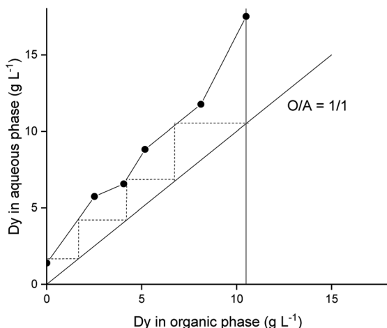
Fig. 5 McCabe–Thieler diagram for the stripping of dysprosium from a loaded organic phase (40 wt% Cyanex 923, 60 wt% [C101][SCN], 11 g L -1 Dy(III)). CaCl 2 in the aqueous phase = 1.0 M. Phase contact time: 60 min, O : A ratios varied between 0.5 : 5 and 5 : 1.5.
