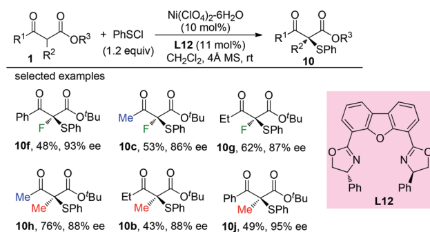
Scheme 60 Ni-Complex catalyzed asymmetric \alpha -sulfonylation.
