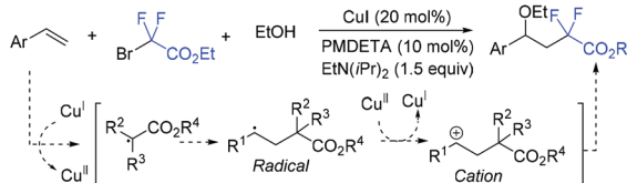
Scheme 46 The difluoroalkylation–thiolation of alkenes with \text{BrCF}_2\text{CO}_2\text{Et} and alcohols.
