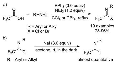
Scheme 1 The preparation of trifluoroacetimidoyl halides.
