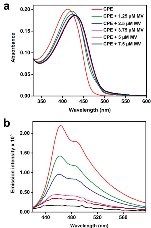
Fig. 2 (a) Absorption and (b) fluorescence spectra ( \lambda_{\text{ex}} = 410 nm) of CPE (5 \mu M, PRU) in water with varying concentrations of MV 2+ as indicated in the figure.
