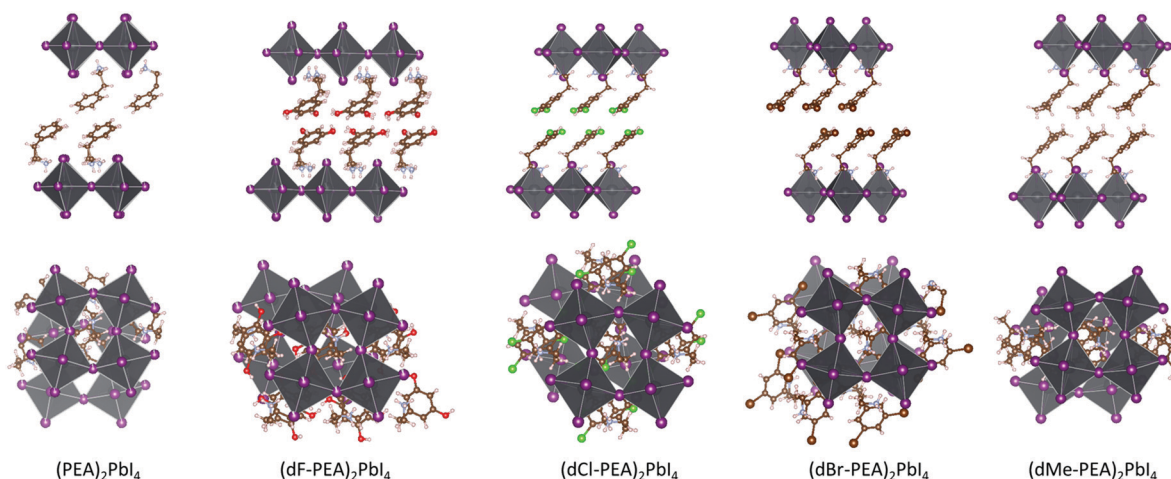
Fig. 2 Crystal structure of (\text{dY-PEA})_2\text{PbI}_4 , Y = H, F, Cl, Br, Me, viewed along the plane of the inorganic sheet and after +90^\circ rotation around the long in-layer axis. The structure of (\text{PEA})_2\text{PbI}_4 is taken from the literature. 34
