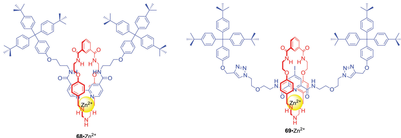
Fig. 29 Ion pair binding [2]rotaxanes.
