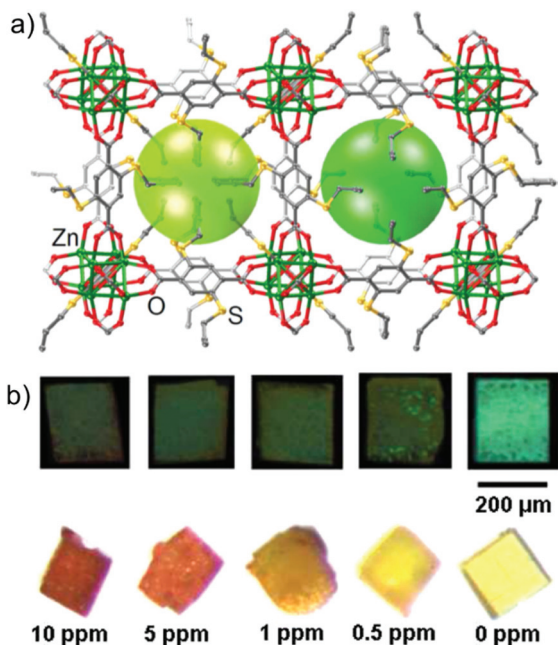
Fig. 6 (a) Single-crystal structure of ASMOF-5. (b) Images of ASMOF-5 crystals under UV-radiation ( \lambda = 365 nm) (top) before and after immersion in \text{Pd}(\text{CH}_3\text{CN})_2\text{Cl}_2 solution in \text{CH}_2\text{Cl}_2 at various concentrations at 80^\circ\text{C} with a duration of immersion of: 1 h (top) and 4 h (bottom). Reproduced with permission from ref. 72. Copyright 2013, American Chemical Society.
