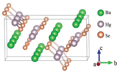
Fig. 25 Crystallographic structure of BaHgSe 2 .
