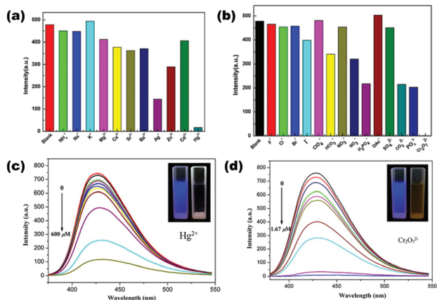
Fig. 8 (a and b) Quenching effect on the fluorescence intensity of (57) by various cations/anions in the aqueous phase; (c and d) fluorescence spectra of (57) in the presence of increasing concentration of \text{Hg}^{2+} and \text{Cr}_2\text{O}_7^{2-} . Inset: Visual changes of quenching effect under UV light (365 nm). Reproduced with permission from ref. 110. Copyright 2015 American Chemical Society.
