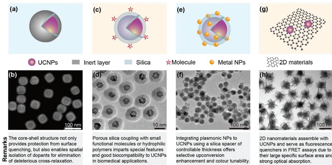
Fig. 3 Strategies of synthesizing and assembling heterogeneous nanostructures. (a) A core-shell structure isolates the dopant ions with the surroundings. (b) HAADF-STEM image of \beta - \text{NaYF}_4 @ \text{NaYbF}_4 :Ho (1 mol%)/@ \text{NaYF}_4 core-shell-shell nanoparticles showing the contrasts between the constituent layers. (c) The design of \text{mSiO}_2 coating for coupling functional molecules to the UCNPs. (d) TEM image of typical \beta - \text{NaGdF}_4 :Yb/Er/Ca@ \text{NaYbF}_4 :Ca@ \text{NaNdF}_4 :Gd/Ca @ \text{mSiO}_2 nanoparticles. (e) The schematic of using silica shell as a spacer for coupling metal nanoparticles to the UCNPs. (f) TEM image of \beta - \text{NaYbF}_4 :Tm (1 mol%)/@ \text{SiO}_2 (3.0 nm)/In nanocomposites. (g) The design of 2D layered nanomaterials for constructing FRET systems. (h) TEM image of \text{MnO}_2 -modified \alpha - \text{NaYbF}_4 :Tm (1 mol%)/@ \text{CaF}_2 nanocomposites. Reprinted with permission from ref. 30, 49, 57 and 81. Copyright 2016 and 2018 American Chemical Society, 2019 WILEY-VCH Verlag GmbH & Co., and 2018 the Royal Society of Chemistry, respectively.
