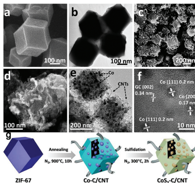
Fig. 13 Morphological and structural features of the ZIF-67 precursor and the \text{Co-C/CNT} intermediate. SEM and HRTEM images of (a and b) ZIF-67 and (c–f) \text{Co-C/CNT} . The lattice fringes highlighted in (f) are in good agreement with the JCPDS reference card no. 15-0806 for metallic cobalt and the characteristic (002) interlayer spacing for graphitic carbon. (g) Schematic drawing of the formation process to obtain the \text{CoS}_2 -C/CNTs nanocomposite. Adapted with permission from ref. 93. Copyright (2018) American Chemical Society.
