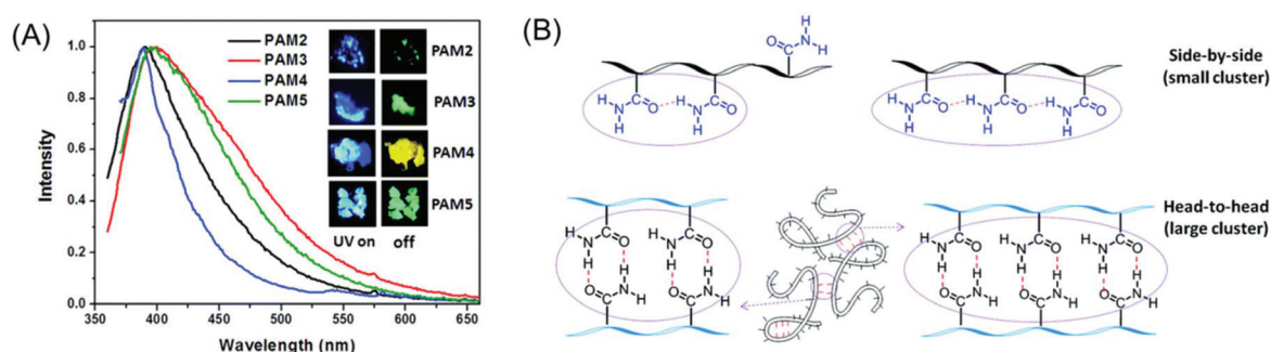
Fig. 21 (A) Prompt fluorescence (λ ex = 347 nm) response of polyacrylamides (PAM2–PAM5). The inset shows their afterglow images while the 365 nm UV source was switched off. (B) Schematic representation demonstrating two different orientations of the polymer chain of PAMs: small and large clusters were formed by intra- and inter-molecular hydrogen bonding, respectively. Reprinted with permission from ref. 115. Copyright (2020), Royal Society of Chemistry.
