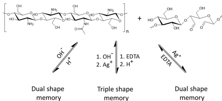
Fig. 8 Schiff base bonds in the triple shape memory gel hydrogel reported by Chen and co-workers respond to pH and \text{Ag}^+ ions. 158
