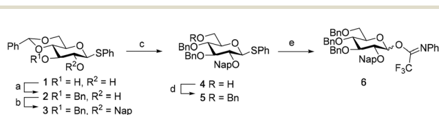
Scheme 1 Synthesis of donor 6 . (a) (i) \text{Bu}_2\text{SnO} , toluene, 120 °C; (ii) \text{CsF} , \text{BnBr} , 76%. (b) \text{NapBr} , \text{NaH} , DMF, 91%. (c) \text{BF}_3 \cdot \text{Et}_2\text{O} , TES, DCM. (d) \text{BnBr} , \text{NaH} , DMF, 88%. (e) (i) NIS, acetone/ \text{H}_2\text{O} (10 : 1, v : v); (ii) 2,2,2-trifluoro- N -phenylacetimidoyl chloride, \text{Cs}_2\text{CO}_3 , acetone, 81% (over two steps).
