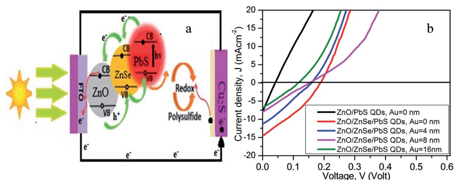
Fig. 6 (a) Electron–hole transport mechanism [ref. 58], and (b) the J – V characteristics of the glass/FTO/ZnO/PbS QDs (black line) and ZnO/ZnSe NRA density varying glass/FTO/ZnO/ZnSe NRs/PbS QD solar cells.
