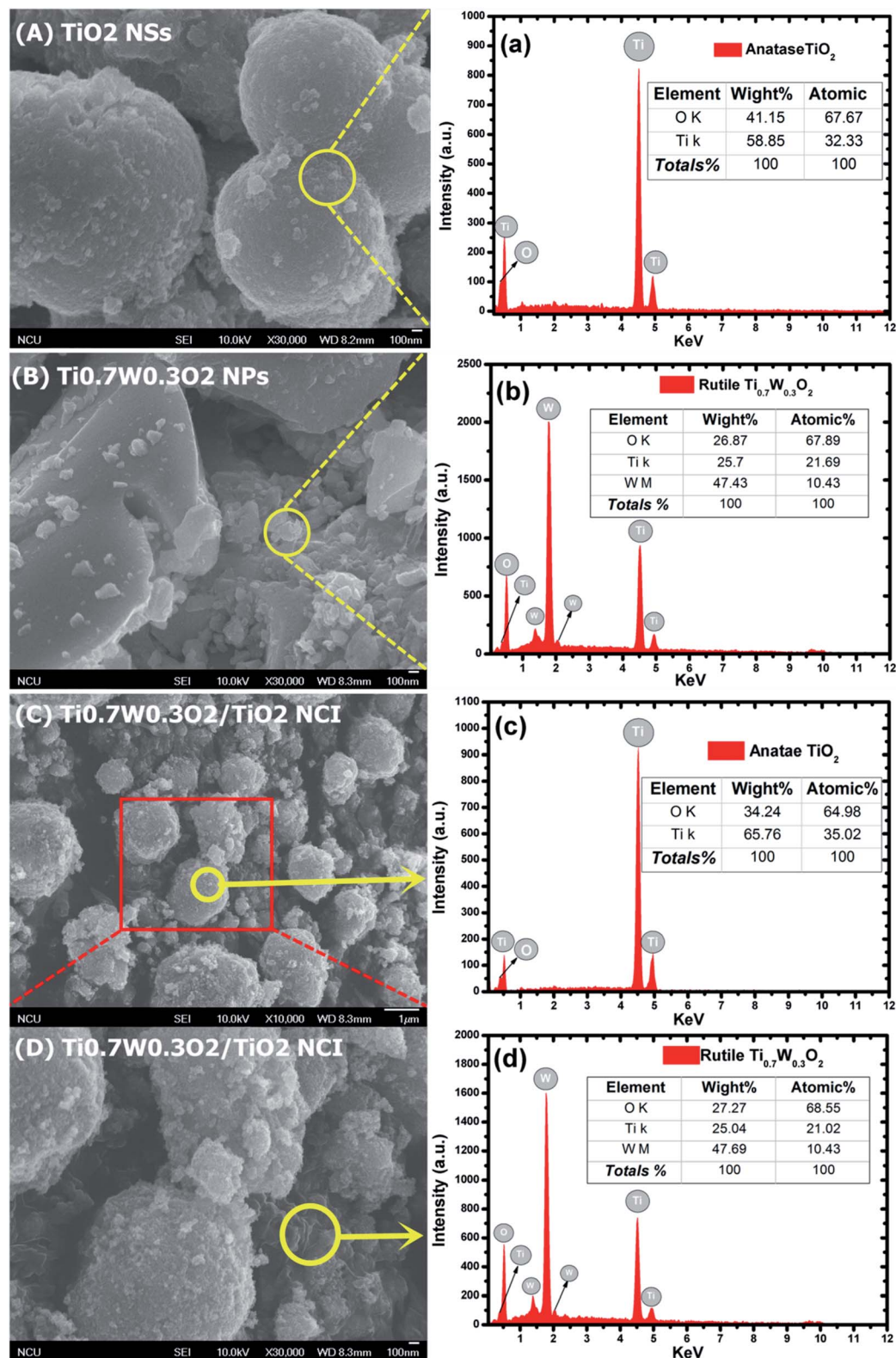
Fig. 2 SEM images of: (A) anatase \text{TiO}_2 , (B) \text{Ti}_{0.7}\text{W}_{0.3}\text{O}_2 and (C)/(D) 5 wt% \text{Ti}_{0.7}\text{W}_{0.3}\text{O}_2/\text{TiO}_2 NCI. The corresponding EDX test results of: (a) anatase \text{TiO}_2 , (b) \text{Ti}_{0.7}\text{W}_{0.3}\text{O}_2 and (c) and (d) 5 wt% \text{Ti}_{0.7}\text{W}_{0.3}\text{O}_2/\text{TiO}_2 NCI, respectively.
