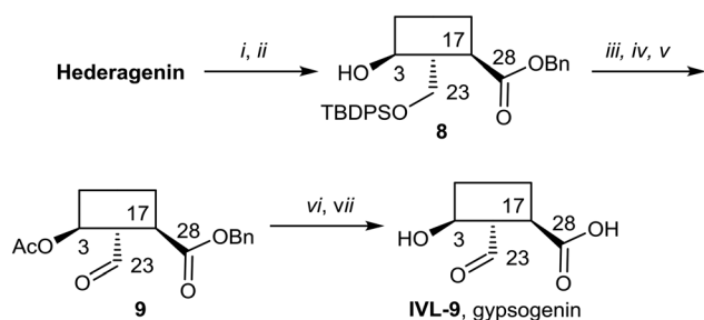
Scheme 6 i. \text{BnBr} , \text{K}_2\text{CO}_3 , \text{DMF} , 25^\circ\text{C} , 75% (S1); ii. TBDSO, imidazole, \text{DCM} , 0^\circ\text{C} to rt, quant. (S1); iii. \text{Ac}_2\text{O} , pyridine, \text{DCM} , rt to 90^\circ\text{C} , 95%; iv. TBAF/ \text{AcOH} , \text{THF} , 50^\circ\text{C} to 100^\circ\text{C} , 27%; v. TEMPO, BAIB, \text{DCM} , 67%; vi. \text{NaOH} , \text{DME}/\text{THF}/\text{H}_2\text{O} , 25^\circ\text{C} , 83%; vii. \text{Pd}(\text{OH})_2/\text{C} , \text{H}_2 , \text{MeOH}/\text{EtOAc} , 80%.
