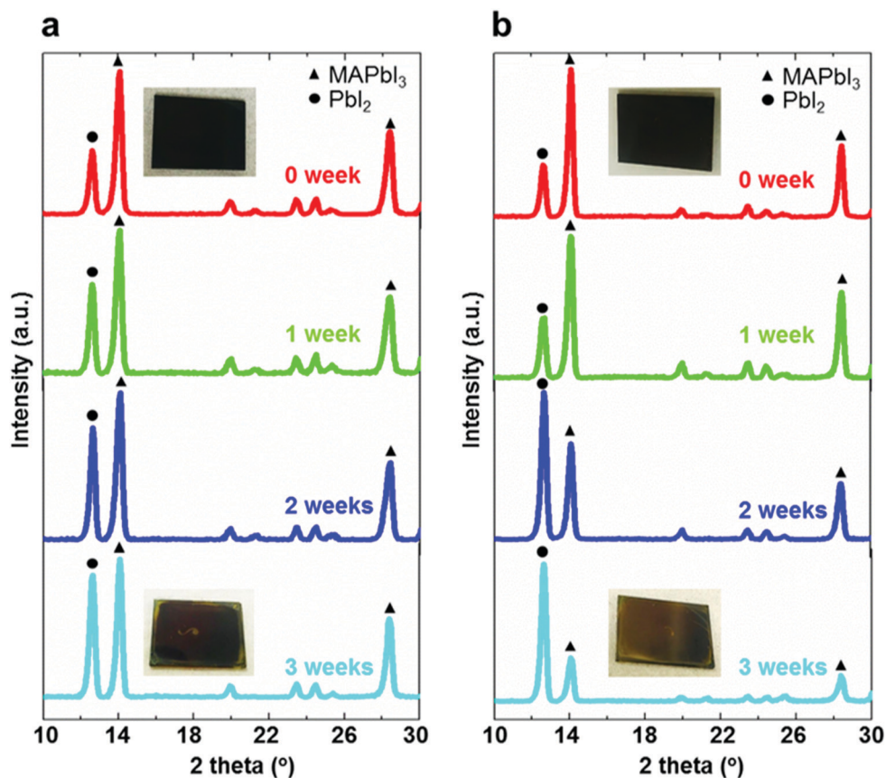
Fig. 3 XRD spectra in the 2\theta range from 10^\circ to 30^\circ of the perovskite films based on (a) the bilayer mesoporous scaffold and (b) the single mesoporous scaffold after different aging times in ambient air at >65% relative humidity. The insets are the top views of the corresponding perovskite films.
