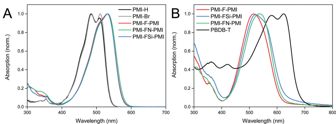
Fig. 2 (A) Optical absorption spectra of PMI, PMI-Br (2), PMI-F-PMI (3a), PMI-FSi-PMI (3b) and PMI-FN-PMI (3c) in solution (chloroform); (B) thin film absorption spectra of PMI-F-PMI (3a), PMI-FSi-PMI (3b), PMI-FN-PMI (3c) and PBDB-T.
