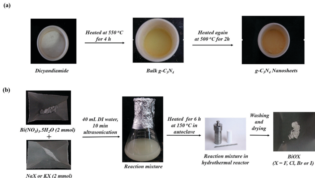
Scheme 1 Schematic representation of the synthesis of (a) \text{g-C}_3\text{N}_4 and (b) hydrothermal synthesis of \text{BiOX} (X = F, Cl, Br and I).
