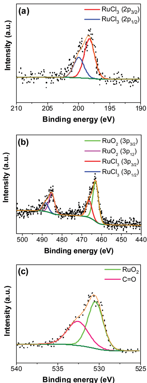
Fig. 5 Fitted HR-XPS of the RuO 2 -CNF electrode surface prepared at 250 °C (a) Cl 2p, (b) Ru 3p, and (c) O 1s. Black dots, olive and orange line represents, experimental data, background and fitted data respectively.
