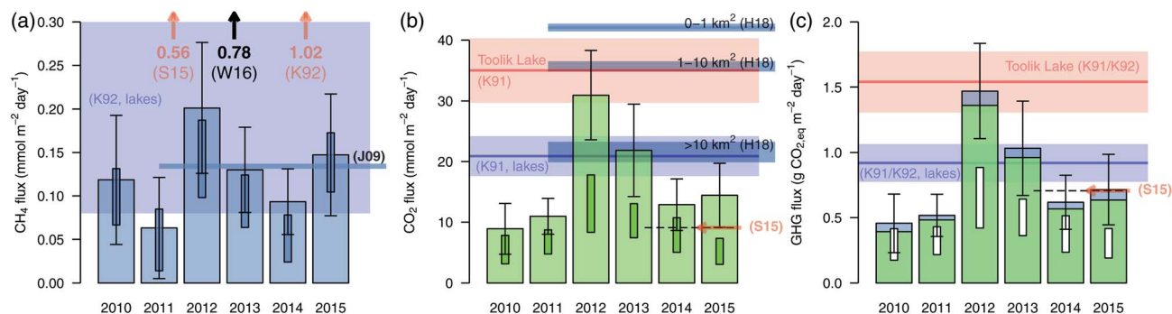
Fig. 11 Average daily fluxes of (a) \text{CH}_4 , (b) \text{CO}_2 , and (c) global warming potential (in \text{CO}_2 -equivalents) during each ice-free periods 2010–2015 of Toolik Lake. Bars show the ice-free mean with standard deviation as vertical whiskers. The darker boxes show the inter-quartile ranges (first to third quartile) of daily medians shown in Fig. 8 and 9, and their median is shown as a white circle. The bluish and reddish bold lines (mean values) and color bands ( \pm SD) show the ranges given by Kling et al. (K91) 5 for Toolik Lake (red color) and (K92) 60 for all lakes (blue color). The more recent estimates for Toolik Lake presented by Sepulveda et al. (S15) 61 (orange arrows; diffuse flux only, because we did not observe ebullition) and a \text{CH}_4 flux estimate by Wik et al. (W16) 45 (black arrow; diffuse flux only for glacial and post-glacial lakes north of 50°N) are also shown for reference. The global estimate of \text{CH}_4 fluxes of Juutinen et al. (J09), 74 and the \text{CO}_2 flux estimates of all boreal lakes from Hastie et al. (H18) 66 are shown with dark blue bars. H18 presents estimates for small ( \leq 1 \text{ km}^2 ), middle (1–10 \text{km}^2 ; Toolik Lake size class), and large lakes ( > 10 \text{ km}^2 ), which are shown separately in panel (b). An additional earlier \text{CH}_4 flux estimation is available from 14 July 1990 (red K92), 60 which is far outside the range presented in panel (a).
