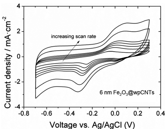
Fig. 7 Cyclic voltammograms of 6 nm Fe 2 O 3 @wpCNTs at scan rates from 10 to 150 mV s -1 .
