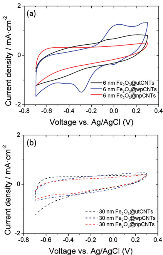
Fig. 6 Areal capacitance of carbon nanotubes with and without plasma treatment, covered with 6 and 30 nm thickness ALD-iron oxide at a 50 mV s -1 scan rate.
