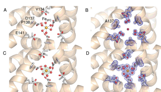
Fig. 2 The 3-fold channel of SynFtn . The channels of wild type (PDB entry 6GKA) (A), variant D137A (B) and variant E62A (C, D) SynFtn viewed along the symmetry axis located at the center of the channel. In each case crystals from which the diffraction data were collected were soaked in a 5 mM Fe 2+ -containing solution for 20 min prior to freezing. Carbon is shown in white, nitrogen in blue, oxygen in red and iron as bright orange spheres with associated water molecules as red spheres. In panels (B) and (D) the blue mesh shows the double difference Fourier (2mF o -DF c ) map contoured at 1.1 σ, while in panel (C) the light green mesh shows the anomalous difference Fourier map calculated from data collected at the iron K-edge and contoured at 10 σ.
