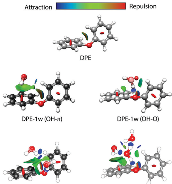
Fig. 7 Non-covalent interaction (NCI) analysis for DPE and its experimentally observed complexes with one water (OH- \pi and OH-O isomers), two water (2w, OH-O structure, compare Fig. 4), and three water (3w) molecules. The structures of DPE-1w and DPE-2w are made transparent to show the experimental atom positions of carbon and oxygen determined from the r_0 fit (for DPE-1w OH- \pi ) and the r_s structure (for DPE-1w OHO and DPE-2w). Blue and green colors identify the presence of hydrogen bonding (strong attraction, blue) and van der Waals interactions (weak attraction, green). Red indicates repulsive interactions.
