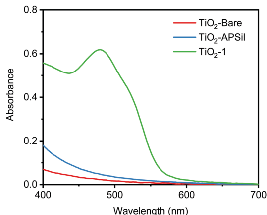
Fig. 1 UV-vis spectra comparing the solid-state absorption spectra of \text{TiO}_2 -Bare, \text{TiO}_2 -APSiI and \text{TiO}_2 -1.
