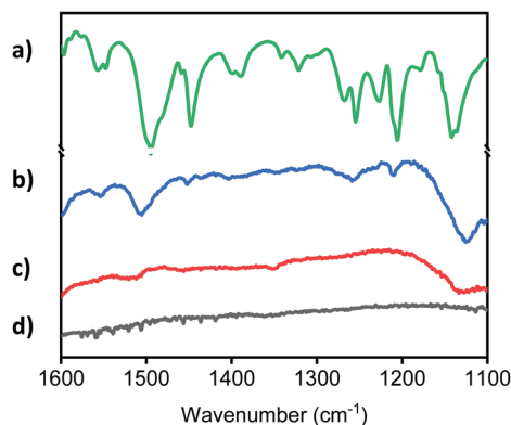
Fig. 2 ATR-FTIR spectra of (a) Sudan I, (b) \text{TiO}_2 -1, (c) \text{TiO}_2 -APSiI, and (d) \text{TiO}_2 -Bare. Spectra (b) through (d) were rescaled, to the same degree, in order to more easily compare their features with the powder sample, (a).
