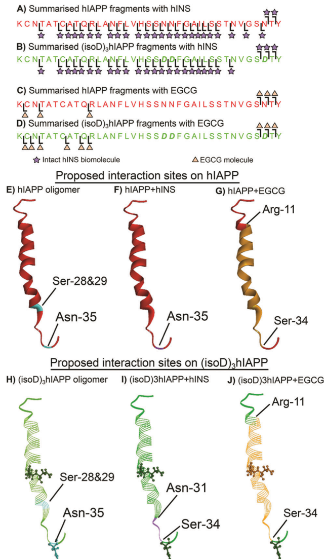
Fig. 2 Summarised fragments of hIINS attached to (A) hIAPP and (B) (isoD) 3 hIAPP. Summarised fragments of EGCG attached to (C) hIAPP and (D) (isoD) 3 hIAPP. The proposed interaction sites on (E) pure hIAPP (PDB 2KB8) 21 with (F) hIINS and (G) EGCG. The proposed interaction sites on (H) pure (isoD) 3 hIAPP with (I) hIINS and (J) EGCG.
