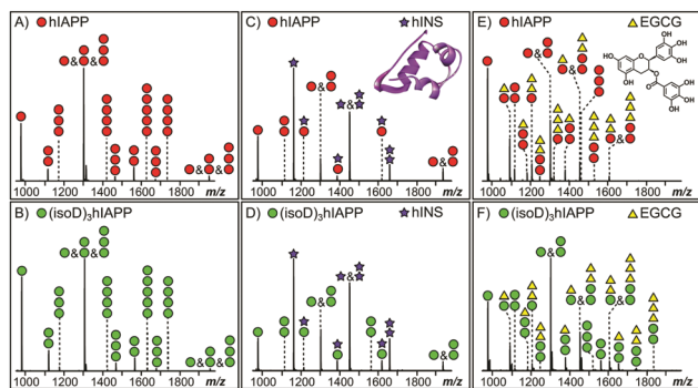
Fig. 1 The MS spectra of the 10 \mu M solutions hIAPP (A; red circle) and (isoD) 3 hIAPP (B; green circle) only, the 10 \mu M solutions of (C) hIAPP and (D) (isoD) 3 hIAPP mixed with 10 \mu M hIINS (purple star); the 10 \mu M solutions of (E) hIAPP and (F) (isoD) 3 hIAPP mixed with 10 \mu M EGCG (yellow triangle).
