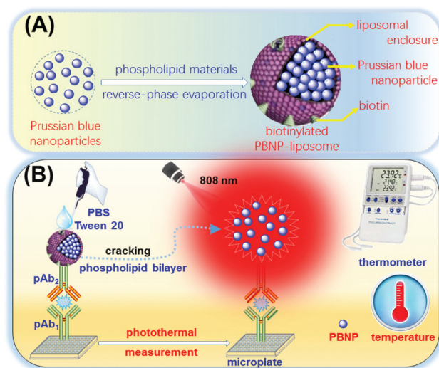
Scheme 1 Schematic illustration of the photothermal immunoassay for neuron-specific enolase (NSE): (A) architectural diagram of the biotinylated liposomes encapsulated with Prussian blue nanoparticles (PBNPs) and (B) photothermal measurement on the anti-NSE primary antibody-coated plate with a sandwiched immunoreaction format using biotinylated PBNP-liposomes as the photothermal conversion material on a portable digital thermometer under 808 nm near-infrared laser irradiation.
