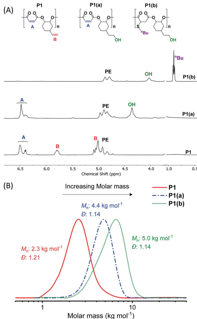
Fig. 1 (A) Selected regions of the ^1H NMR spectra showing the changes in proton resonances of (purified) polymers after functionalization steps (in DMSO-d_6 ). (B) SEC (in DMF) showing an increase in molar mass after functionalization, in each case with retention of monomodal distributions and narrow dispersity (see ESI† for more details).
