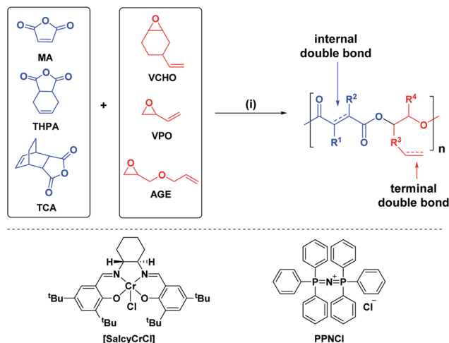
Scheme 2 ROCOP of the series of epoxides and anhydrides. Reagents and conditions (i) [SalicyCrCl] , PPNCI , 60 °C, toluene, molar ratio: [SalicyCrCl]/PPNCI/CHD/anhydride/epoxide = 1/1/10/100/120 , [anhydride] = 5 M.
