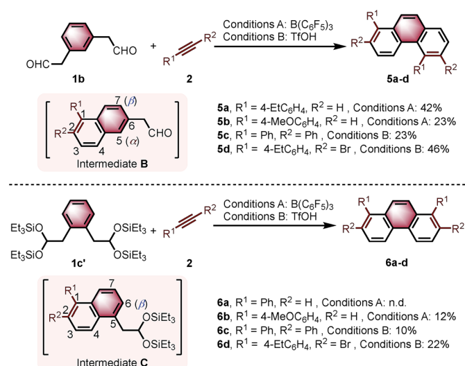
Scheme 4 The reaction of 1b and 1c' with alkynes. Reaction conditions: 1b or 1c' (0.10 mmol), 2 (0.25 mmol). Conditions A: 20 mol% B(C_6F_5)_3 /MS4Å, DCM/HFIP = 10 : 1, rt, 15 h. Conditions B: 150 mol% TfOH, CF_3Ph /HFIP = 10 : 1, -30\text{ }^\circ\text{C} , 15 h. Yields given correspond to isolated yields. n.d. = not detected.
