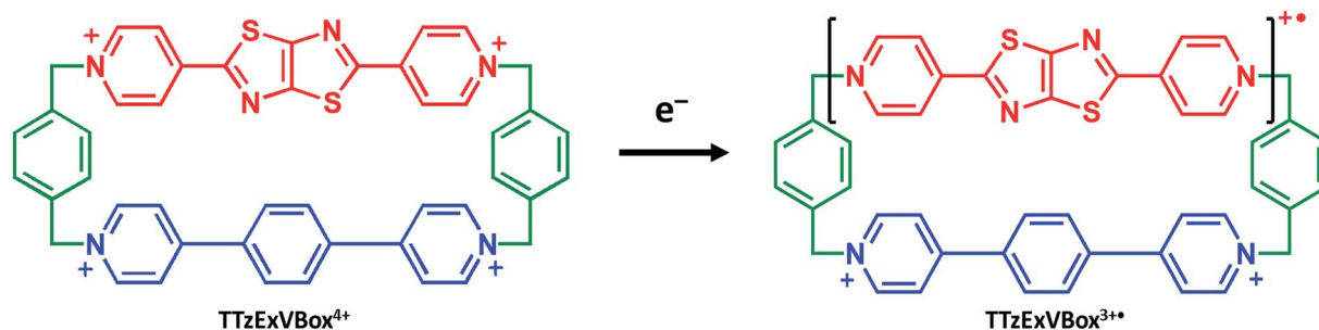
Scheme 1 Chemical reduction of \text{TTzExVBox}^{4+} to \text{TTzExVBox}^{3+\bullet} .
