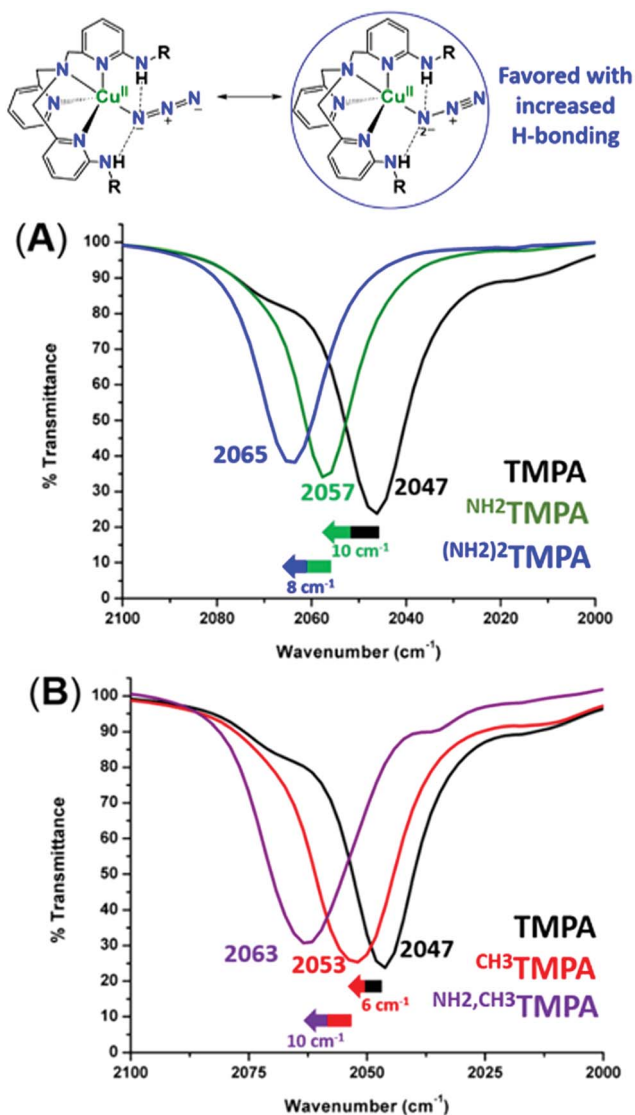
Fig. 3 Infrared spectra of [(X)TMPA)Cu^{II}(N_3^-)]^+ complexes in CH_3CN , showing the increase of the \nu(N-N) stretch upon incorporation of amino substituents (A) and incorporation of steric functionalities (B).
