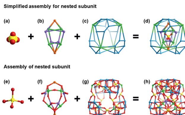
Fig. 1 Simplified (a–d) and real (e and h) three-shell nested subunit for NENU-605 . (a, e) The innermost shell (central PO 4 3- group); (b, f) the shuttle-shaped second shell ({Na 2 K 4 Mn 4 }); (c, g) the cage-like outermost shell (Mn 4 {(P 4 Mo 6 V ) 4 }); (d, h) the overall three-shell nested substructure. Colour code: P yellow, O red, Na orange, K light purple, Mn green, and Mo light blue.
