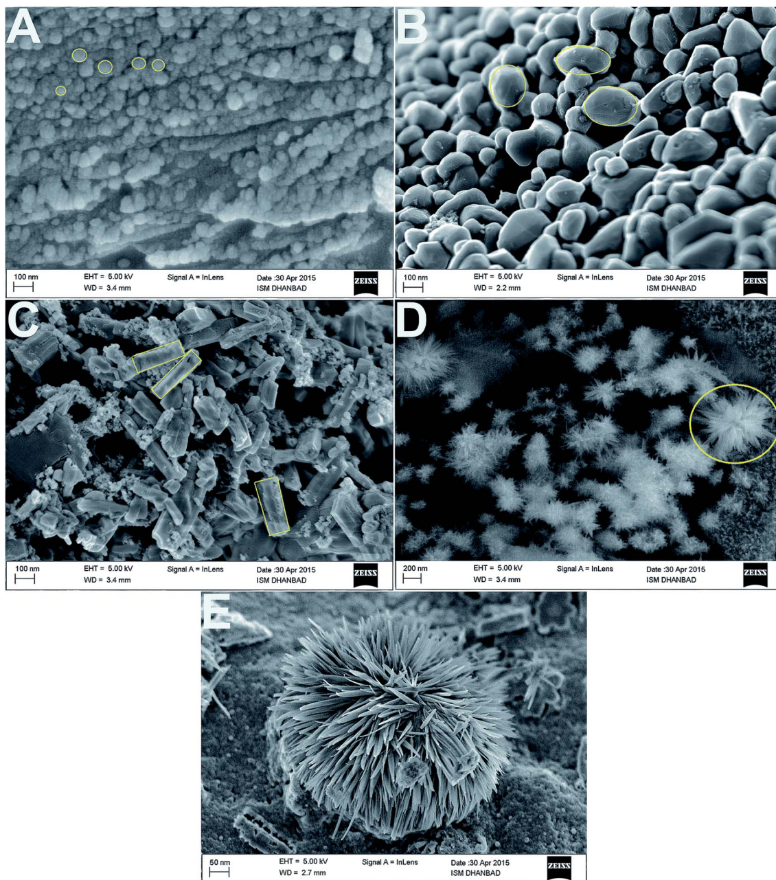
Fig. 12 FE-SEM images of the (A) spherical, (B) oval, (C) rod and (D) flower-shaped silver nanoparticles at low and (E) high magnifications 40b (adapted with permission from Royal Society of Chemistry, 2015).
