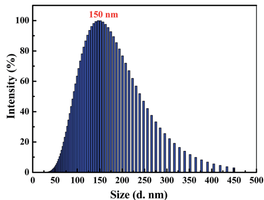
Fig. 2 Size distribution curve of luminogen 1 ( 2.0 \times 10^{-5} mol \text{L}^{-1} ) in acetonitrile–water mixtures with f_w = 90\% .
