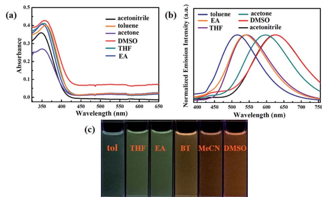
Fig. 3 (a) UV-Vis absorption spectra and (b) normalized fluorescence spectra (Excitation wavelength = 380 nm) of luminogen 1 in different solvents ( 2.0 \times 10^{-5} mol \text{L}^{-1} ). (c) Photographs of 1 under 365 nm UV illumination in different solvents: tol (toluene); THF (tetrahydrofuran); EA (ethyl acetate); BT (acetone); MeCN (acetonitrile); DMSO (dimethyl sulfoxide).
