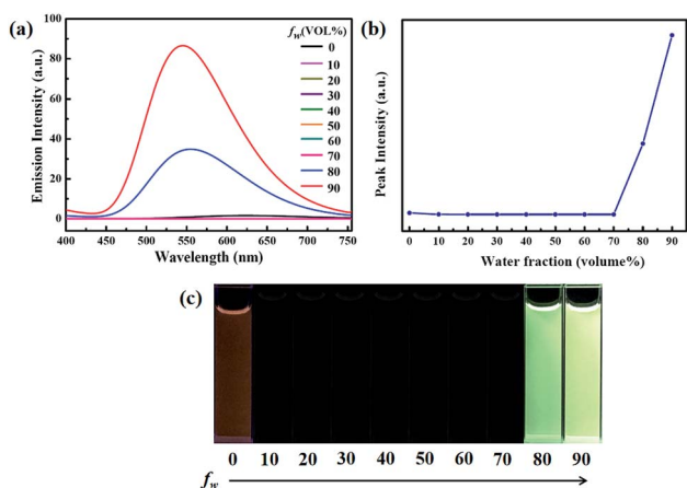
Fig. 1 (a) Fluorescence spectra of the dilute solutions of 1 ( 2.0 \times 10^{-5} mol \text{L}^{-1} ) in acetonitrile–water mixtures with different water content (0–90%). Excitation wavelength = 380 nm. (b) Changes the emission intensity of 1 at 545 nm in acetonitrile–water mixtures with different volume fractions of water (0–90%). (c) PL images of 1 ( 2.0 \times 10^{-5} mol \text{L}^{-1} ) in acetonitrile–water mixtures with different f_w values under 365 nm UV illumination.
