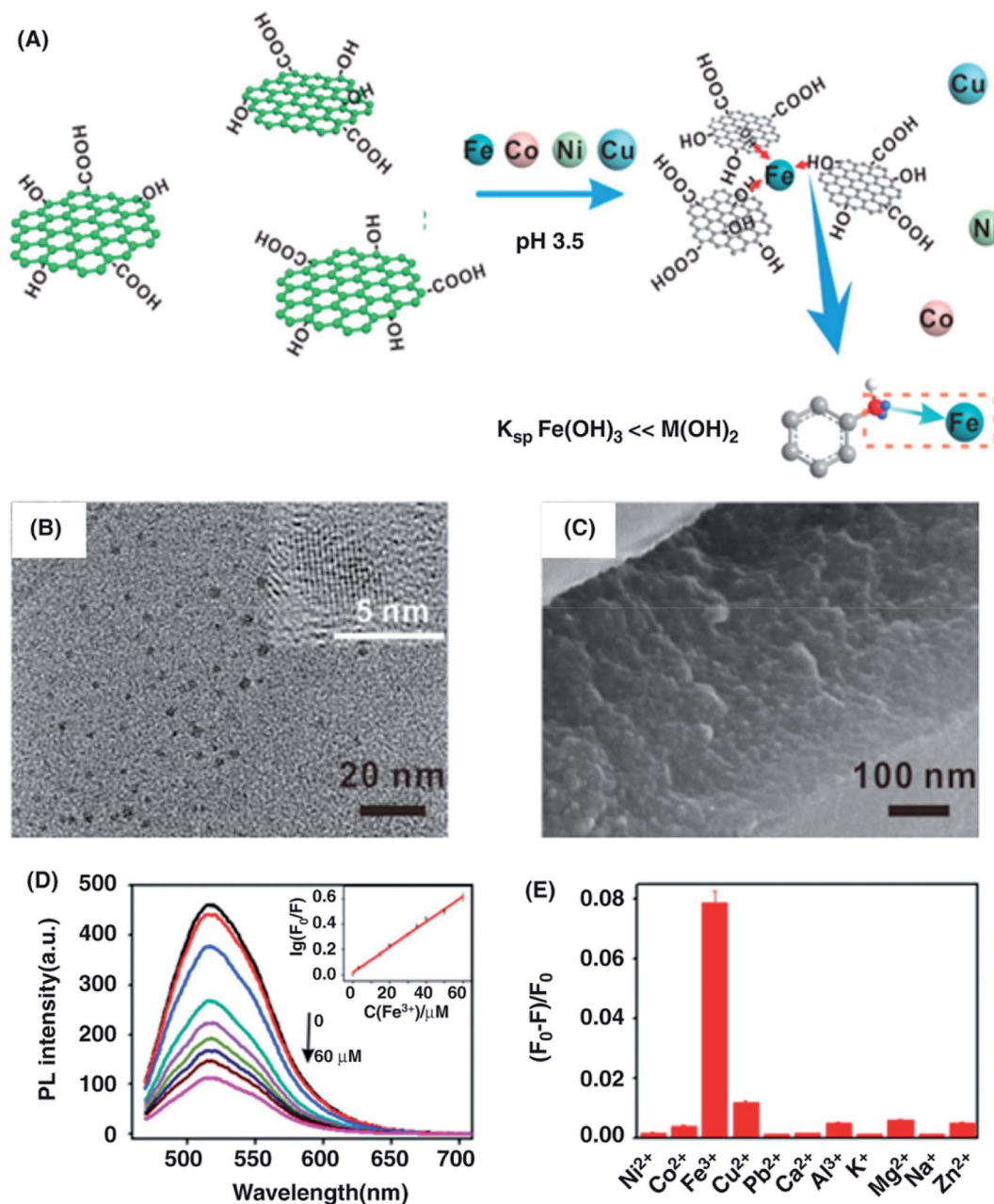
Fig. 36 (A) \text{Fe}^{3+} ions sensing platform showing GQD fluorescence quenching by \text{Fe}^{3+} ions and the selectivity of \text{Fe}^{3+} ions by GQDs among other interfering metal ions. (B) TEM and HETEM images of the GQDs. Inset shows the lattice fringes of GQDs. (C) SEM image of GQD aggregation induced after adding \text{Fe}^{3+} ions. (D) PL intensity of GQDs in different concentrations of \text{Fe}^{3+} ranging from 0 to 60 \mu\text{M} . Inset shows a linear calibration plot for detecting \text{Fe}^{3+} ions. (E) Selectivity of GQDs toward \text{Fe}^{3+} ions over 10 other common interfering metal ions at identical concentrations of 5 \mu\text{M} for all metal ions. [Reprinted with permission from ref. 700, X. Zhu, Z. Zhang, Z. Xue, C. Huang, Y. Shan, C. Liu, X. Qin, W. Yang, X. Chen and T. Wang, Understanding the Selective Detection of \text{Fe}^{3+} Based on Graphene Quantum Dots as Fluorescent Probes: The K_{\text{sp}} of a Metal Hydroxide-Assisted Mechanism, Anal. Chem. , 2017, 89 , 12054–12058. Copyright© American Chemical Society.]
