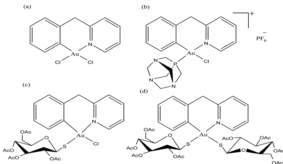
Fig. 29 Chemical structure of novel (\text{C}^{\wedge}\text{N})\text{gold(III)} cyclometallated compounds (a) [\text{Au}(\text{py}^b\text{-H})\text{Cl}_2] , (b) [\text{Au}(\text{py}^b\text{-H})(\text{PTA})\text{Cl}]\text{PF}_6 , (c) [\text{Au}(\text{py}^b\text{-H})(\text{GST})\text{Cl}] and (d) [\text{Au}(\text{py}^b\text{-H})(\text{GST})_2] .
