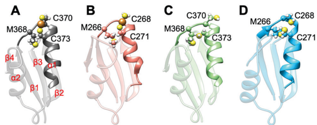
Fig. 4 Structures of the most populated clusters of MBD3/4. (A) Holo MBD4. Secondary structure motifs \alpha 1 , \alpha 2 and \beta 1-4 are labelled. (B) Holo MBD3. (C) Apo MBD4. (D) Apo MBD3. Cu(i) is shown as an orange sphere; sulphur and hydrogen atoms are in yellow and white, respectively. Carbon atoms are shown in the colour scheme of the protein. The Cu loop and \alpha 1 are shown in opaque, whereas the rest of the protein is shown as transparent new cartoon representation.
